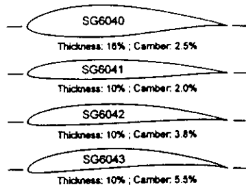
Fig. 1 Contours of the root and primary airfoils
