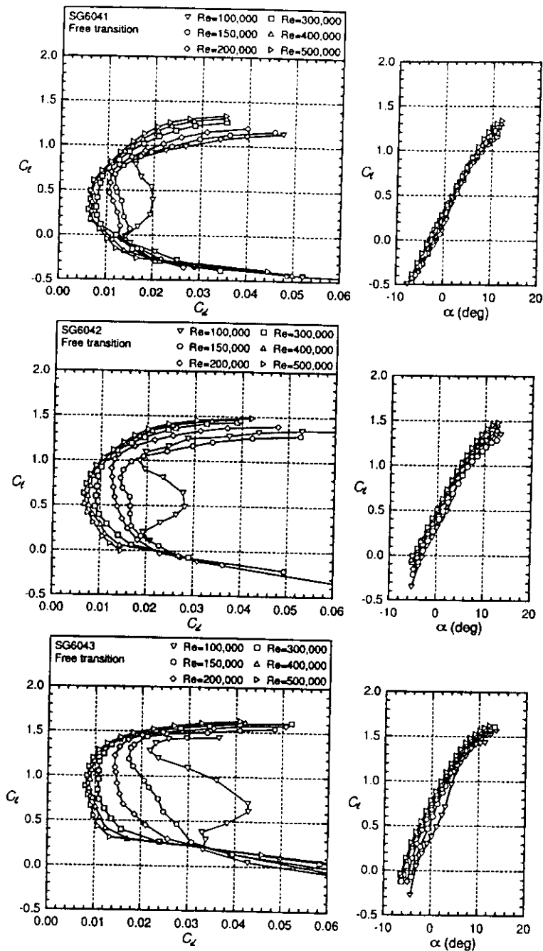
Fig. 4 Drag polars and corresponding lift curves for the SG6041, SG6042, SG6043 primary airfoils (free transition)
