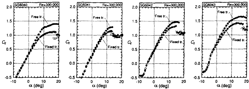
Fig. 7 Lift curves for the root and the primary airfoils at their design Reynolds numbers (free and fixed transition): dark symbols, increasing \alpha and open symbols, decreasing \alpha
