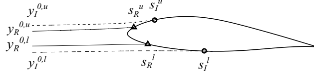
Figure 1. Definition of particle impact and rupture limits.
