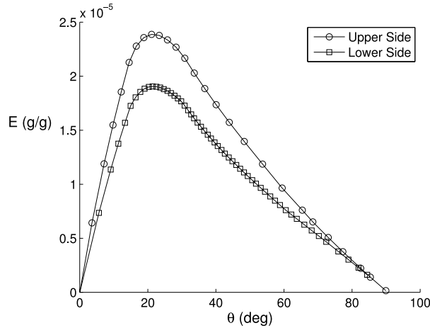
Figure 10. Erosion rate E at r/R = 0.35 , \alpha = 3.5 deg.
