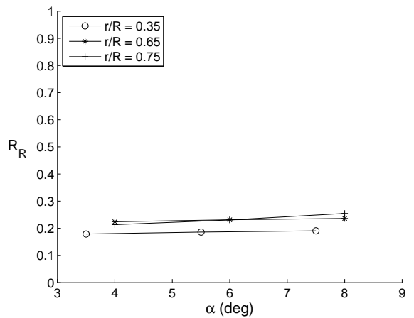
Figure 5. (a) Insect impact surface ratio R_I and (b) rupture surface ratio R_R at three blade spanwise locations.
