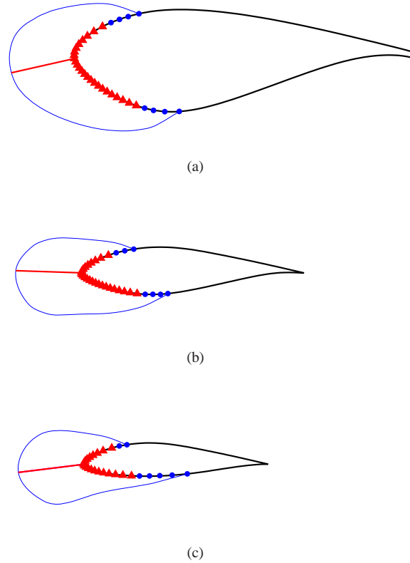
Figure 6. Contours of insect normal impact velocity V_N/V_\infty at (a) r/R = 0.35 ( \alpha = 5.5 deg), (b) r/R = 0.65 ( \alpha = 6 deg), (c) and r/R = 0.75 ( \alpha = 6 deg); circles placed at impingement locations, triangles at rupture locations, and red segments at maximum V_N/V_\infty .
